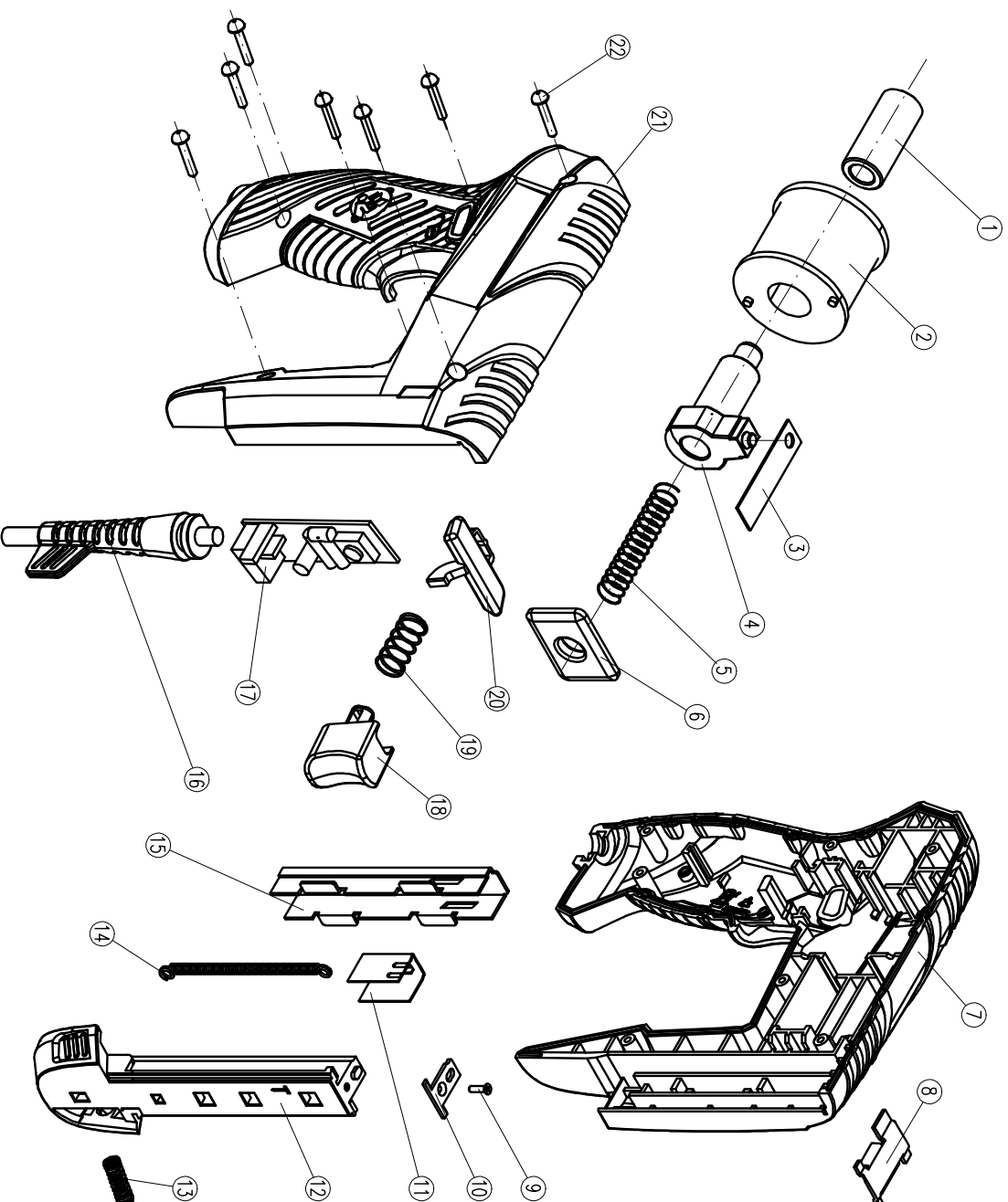
Exploded View for J-119
