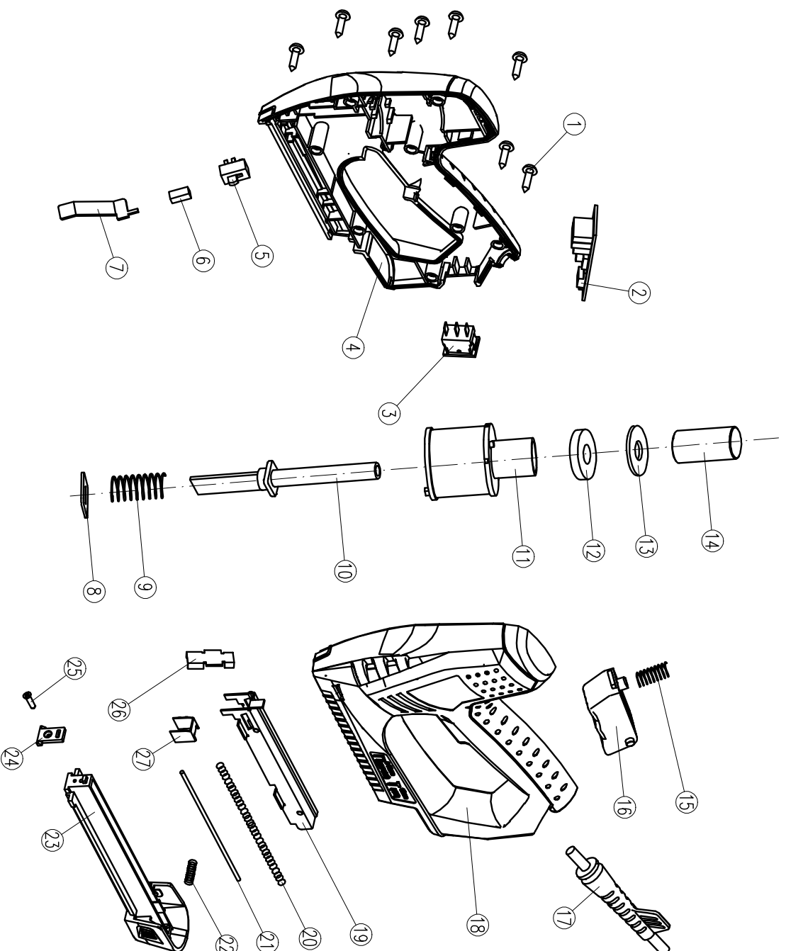
Exploded View for J-123
